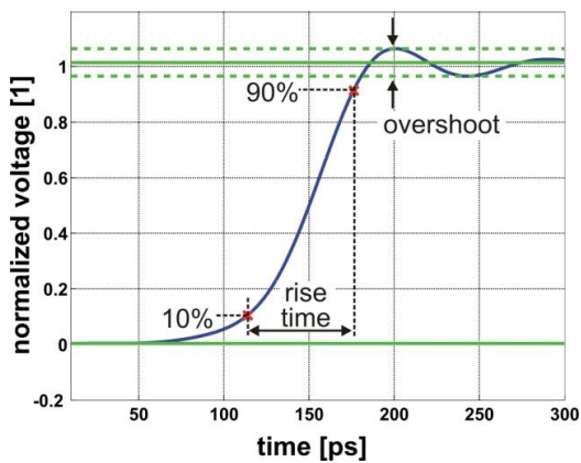
Figure 1: Rise-time and overshoot.
