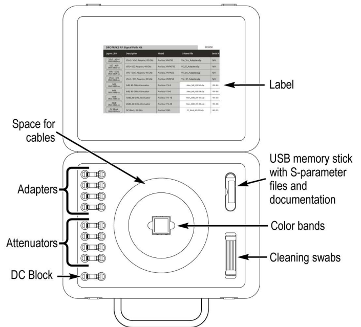
DPO7RFK2-Extended 1.85 mm characterized attenuator/adapter kit.
