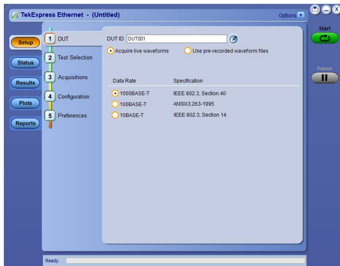
Ethernet Compliance Test Solution (Option CMENET3) - Receive full PHY layer support for Ethernet variants 10BASE-T, 100BASE-TX, and 1000BASE-T with the comprehensive, integrated Tektronix® Ethernet tool set. Analog verification, automated compliance software, and device characterization solutions are all included.
