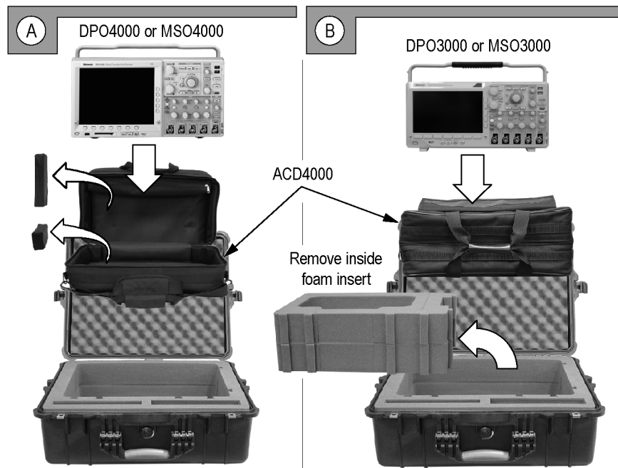
Figure 3: Transit case description; DPO3000, MSO3000, DPO4000, and MSO4000
