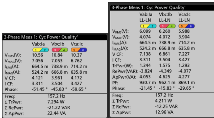
Figure 5: Power quality test results in Line-Line mode (left) and in the Line-Neutral mode (right)
