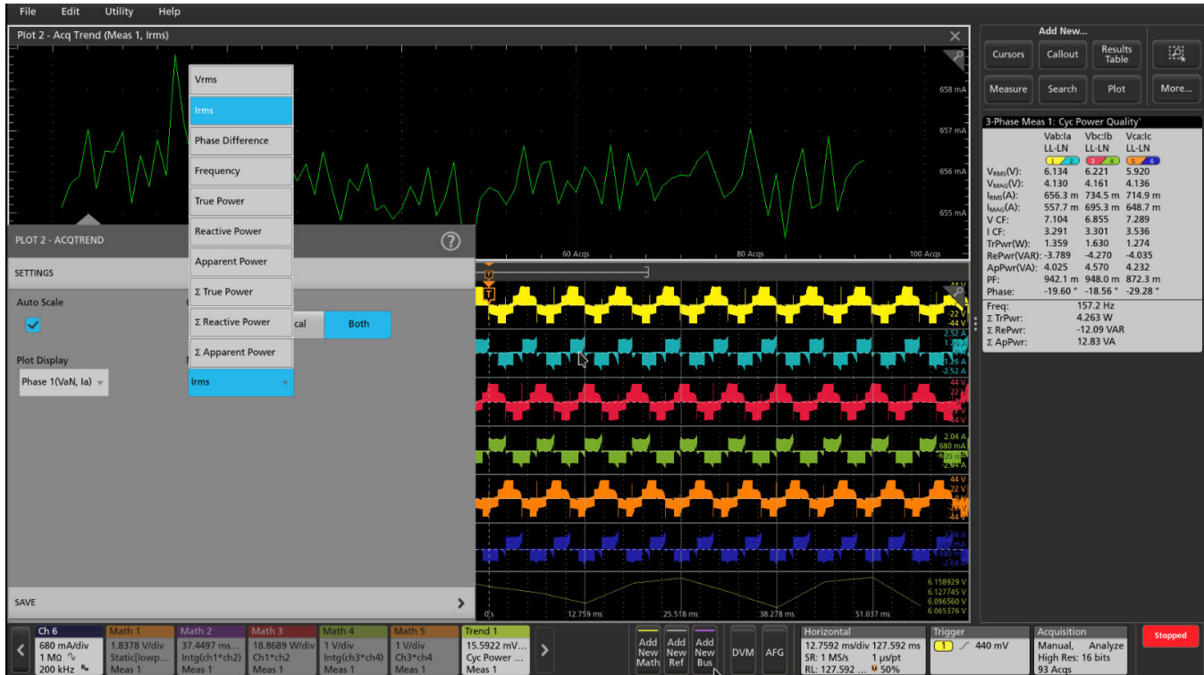
Figure 7: The Acq Trend plot enables user to monitor system behaviour over long records. Choose from a range of parameters of the Power quality measurement to plot the trend data. The Acq Trend of Irms plotted over 93 acquisitions is shown in green.
