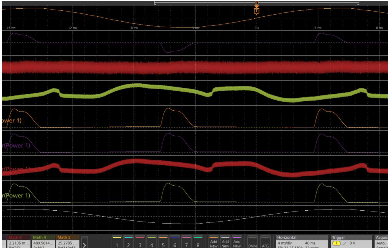
Efficiency measurement
