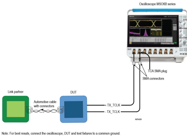
Automotive Ethernet connection diagram
