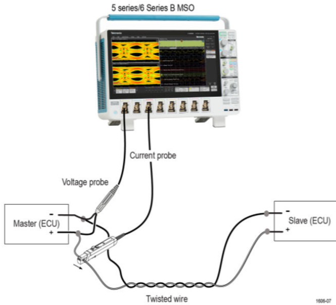
Software based signal separation configuration
