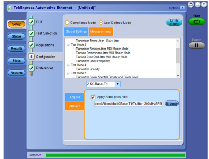
User defined configuration for PSD test
